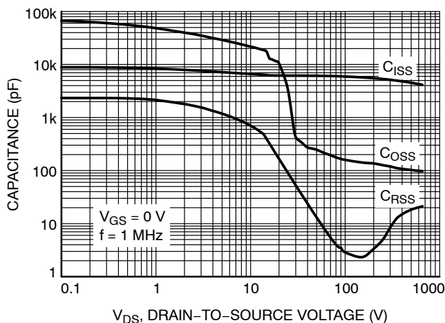
Figure 15. Capacitance Variation
