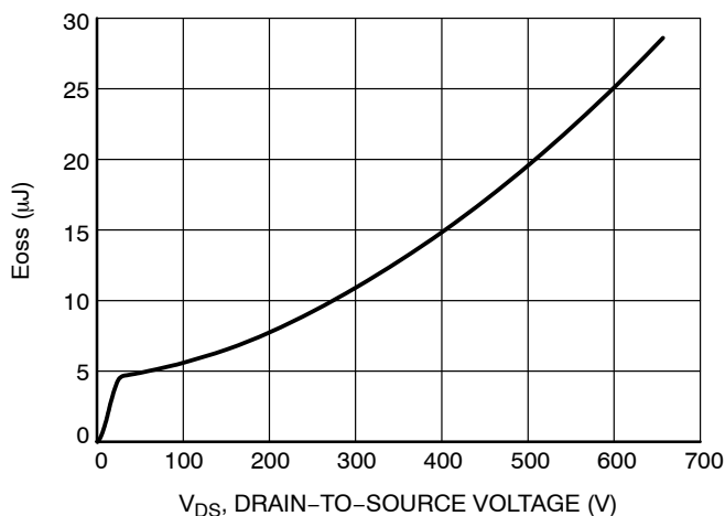
Figure 14. E_{oss} vs. Drain-to-Source Voltage
