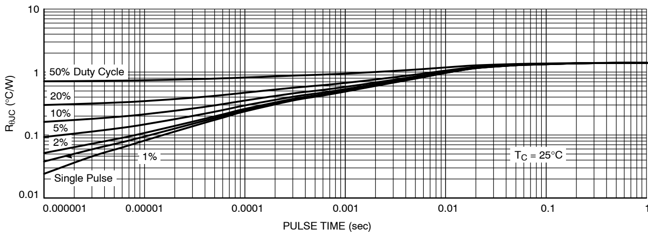
Figure 14. Thermal Characteristics
