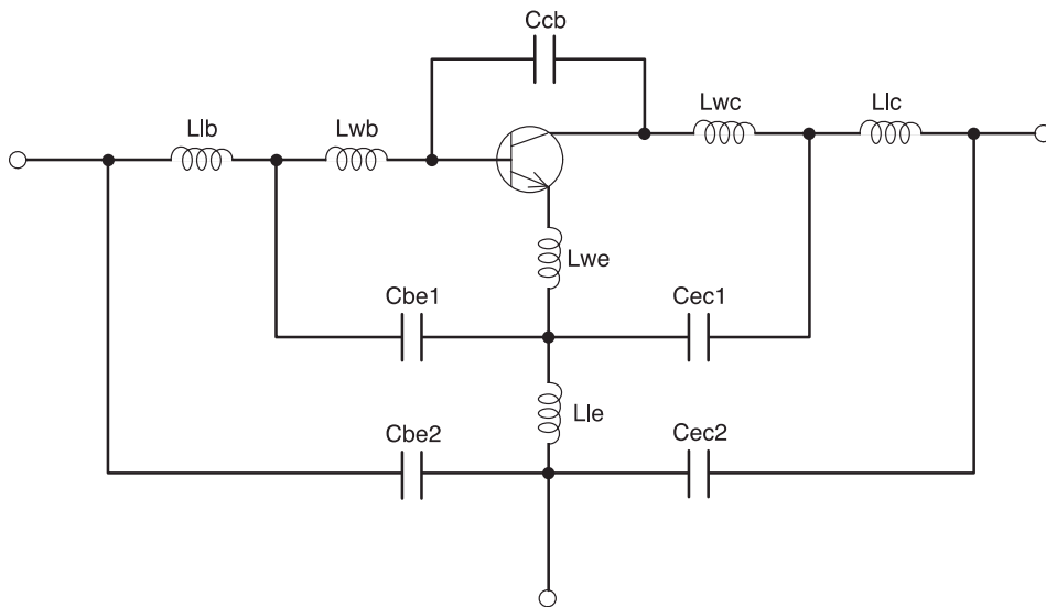
Figure 10. Schematic
