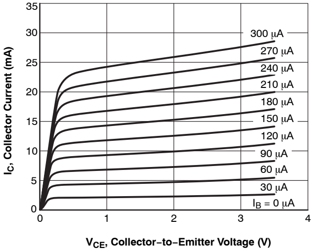
Figure 1. I_C - V_{CE}
