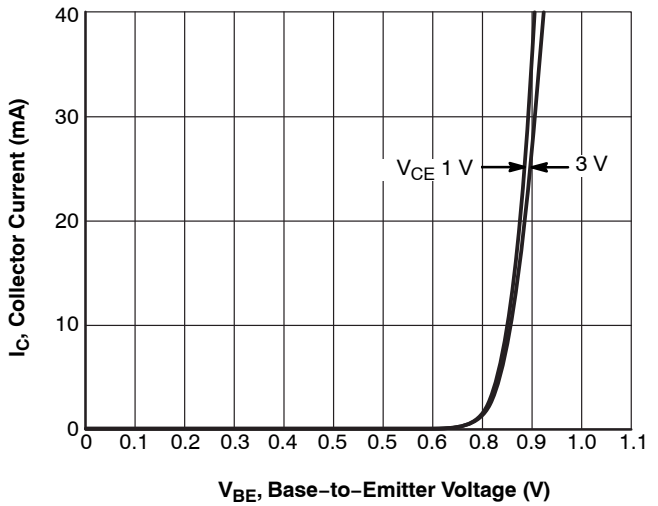
Figure 2. I_C - V_{BE}
