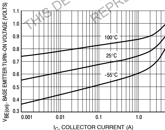
Figure 5. Base Emitter Turn-On Voltage versus Collector Current
