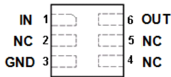
Figure 3. Pin Description
