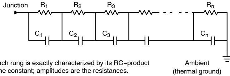
Figure 33. Non-Grounded Capacitor Thermal Ladder (“Foster” Ladder)
