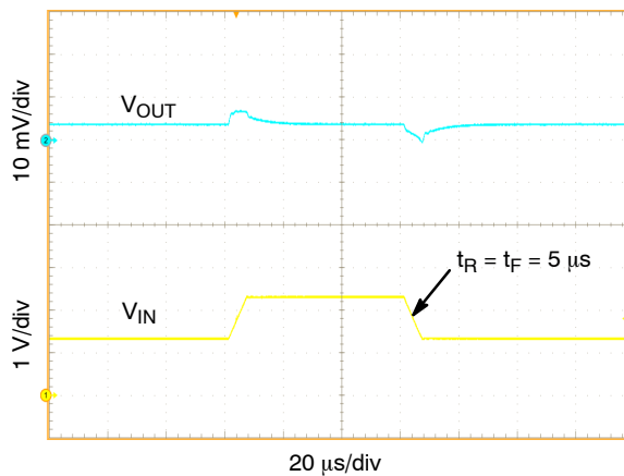
Figure 18. V_{IN} Line Transient Response, V_{IN} = 1.3\text{ V} to 2.3\text{ V} , I_{OUT} = 100\text{ mA} , C_{OUT} = 2.2\text{ }\mu\text{F}
