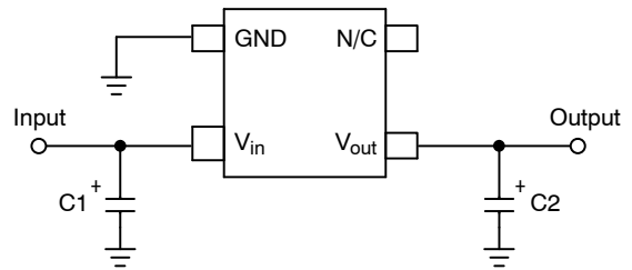
Figure 2. NCP663/NCV663 Typical Application Diagram
