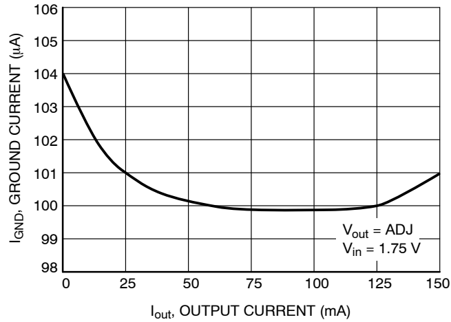
Figure 22. Ground Current vs. Output Current
