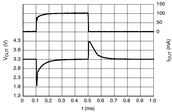
Figure 31. Load Transients, 3.3 V Version, I OUT = 1 – 100 mA, t R = t F = 0.5 μs, V IN = 4.3 V
