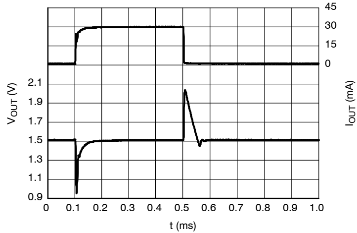
Figure 32. Load Transients, 1.5 V Version, I OUT = 1 – 30 mA, t R = t F = 0.5 μs, V IN = 2.5 V
