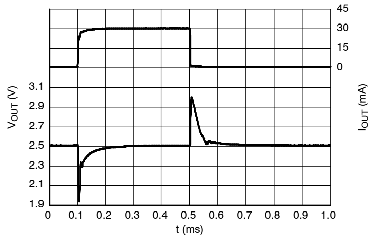
Figure 33. Load Transients, 2.5 V Version, I OUT = 1 – 30 mA, t R = t F = 0.5 μs, V IN = 2.5 V
