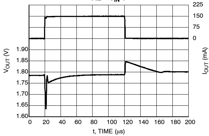
Figure 63. Load Transients, 1.8 V Version, I_{\text{OUT}} = 1 - 150 \text{ mA} , t_{\text{R}} = t_{\text{F}} = 0.5 \mu\text{s} , V_{\text{IN}} = 2.8 \text{ V} , \text{AE} = 0 \text{ V}
