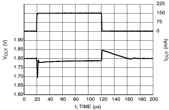
Figure 64. Load Transients, 1.8 V Version, I_{\text{OUT}} = 1 - 150 \text{ mA} , t_{\text{R}} = t_{\text{F}} = 0.5 \mu\text{s} , V_{\text{IN}} = 2.8 \text{ V} , \text{AE} = V_{\text{IN}} \text{ V}
