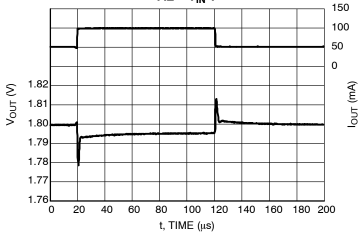
Figure 69. Load Transients, 1.8 V Version, I OUT = 50 - 100 mA, t R = t F = 0.5 μs, V IN = 2.8 V, AE = V IN V
