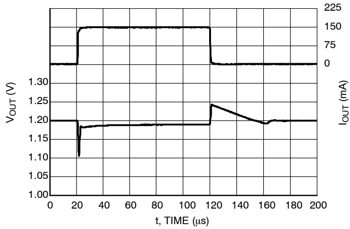
Figure 62. Load Transients, 1.2 V Version, I_{\text{OUT}} = 1 - 150 \text{ mA} , t_{\text{R}} = t_{\text{F}} = 0.5 \mu\text{s} , V_{\text{IN}} = 2.2 \text{ V} , \text{AE} = V_{\text{IN}} \text{ V}
