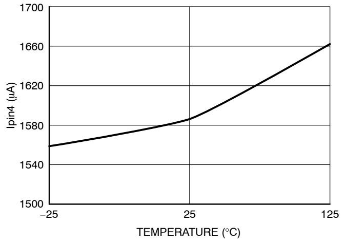
Figure 10. Pin4 Charge Current vs. Temperature (@ Ipin5 = 1.5 mA)
