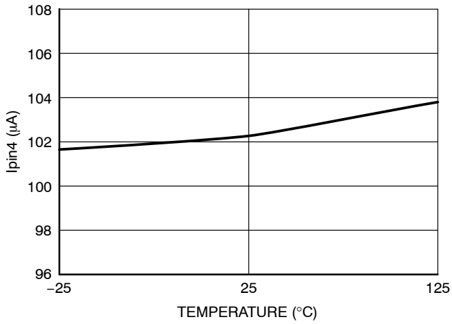
Figure 9. Pin4 Charge Current vs. Temperature (@ Ipin5 = 100 μA)
