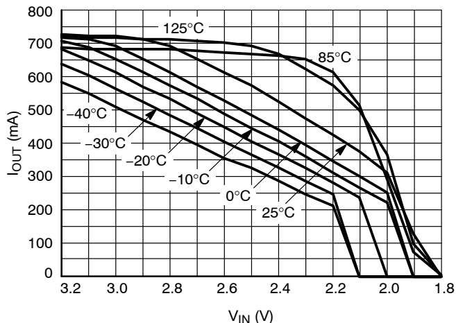
Figure 21. Output Current Capability for the 1.8 V Version
