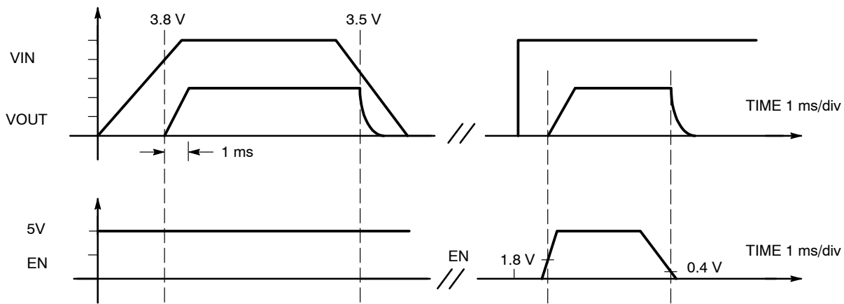
Figure 3. Timing Diagram
