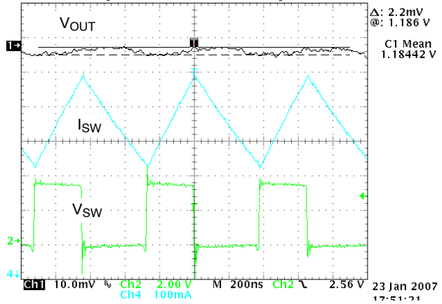
Figure 26. PWM Switching Waveforms (V_{IN} = 3.6\text{ V}, V_{OUT} = 1.2\text{ V}, I_{OUT} = 600\text{ mA}, Temperature = 25°C)
