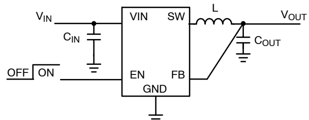
Figure 2. Typical Application for Fixed Version
