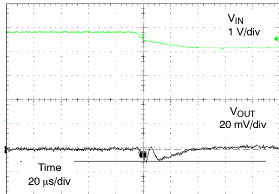
Figure 18. 3.6 V to 3.0 V Line Transient (\text{Risetime} = 50 \mu\text{s}, V_{OUT} = 1.2 \text{ V}, I_{OUT} = 100 \text{ mA}, T_A = 25^\circ\text{C})
