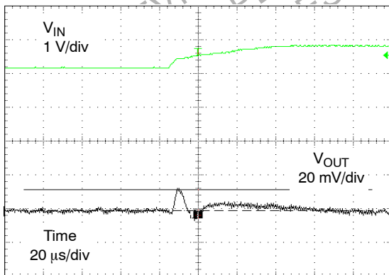
Figure 17. 3.0 V to 3.6 V Line Transient (\text{Risetime} = 50 \mu\text{s}, V_{OUT} = 1.2 \text{ V}, I_{OUT} = 100 \text{ mA}, T_A = 25^\circ\text{C})
