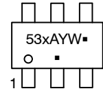
TSOP-6 CASE 318G STYLE 13
