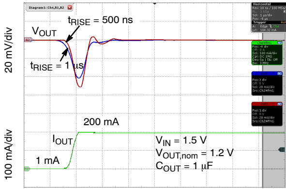
Figure 33. Load Transient Response, I_{OUT} = 1 \text{ mA to } 200 \text{ mA}
