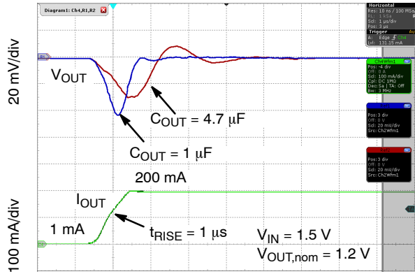
Figure 31. Load Transient Response, I_{OUT} = 1 \text{ mA to } 200 \text{ mA}
