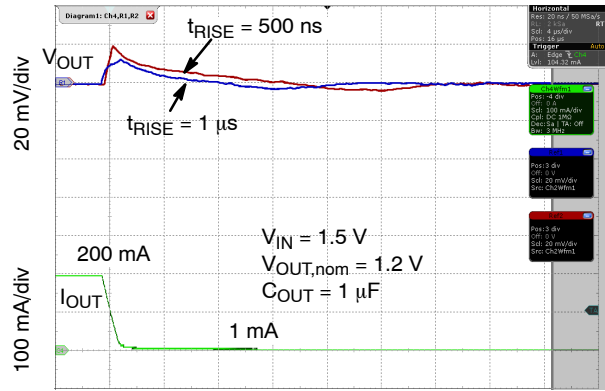
Figure 34. Load Transient Response, I_{OUT} = 1 \text{ mA to } 200 \text{ mA}
