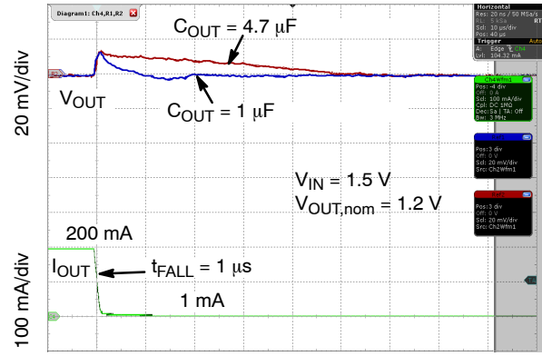
Figure 32. Load Transient Response, I_{OUT} = 1 \text{ mA to } 200 \text{ mA}
