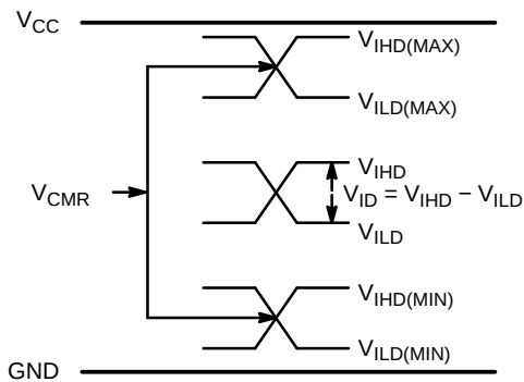
Figure 14. V_{CM} Diagram
