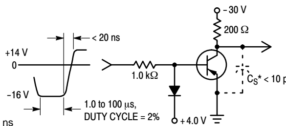
Figure 2. Turn–Off Time
