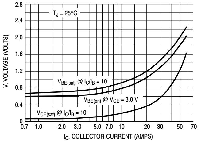
Figure 8. "On" Voltages
