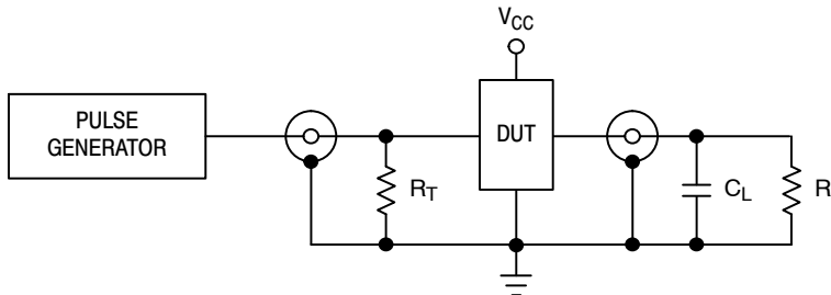
Figure 3. AC Waveforms
