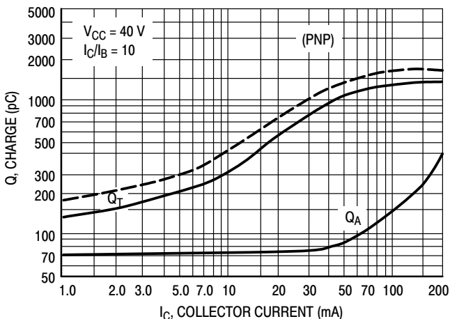
Figure 23. Charge Data
