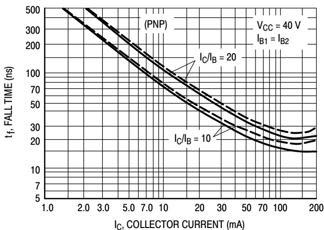
Figure 25. Fall Time
