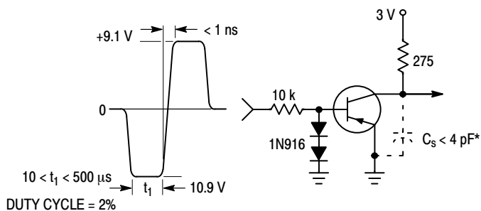
Figure 21. Storage and Fall Time Equivalent Test Circuit
