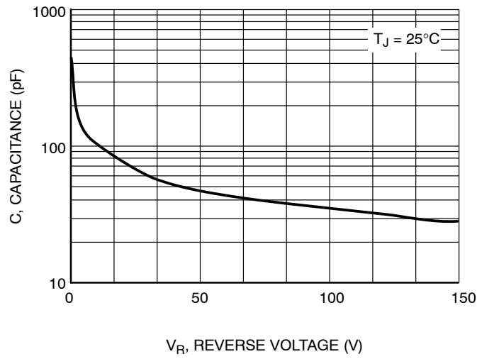
Figure 7. Capacitance
