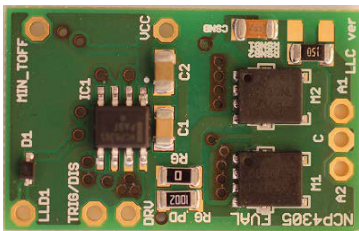
Figure 8. Evaluation Board Photo – Top Side
