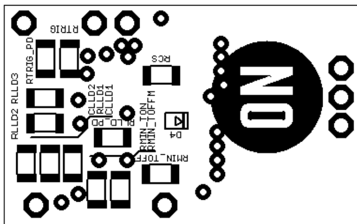
Figure 7. Bottom Side Components
