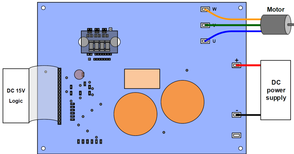
Figure 5. Connection Example
