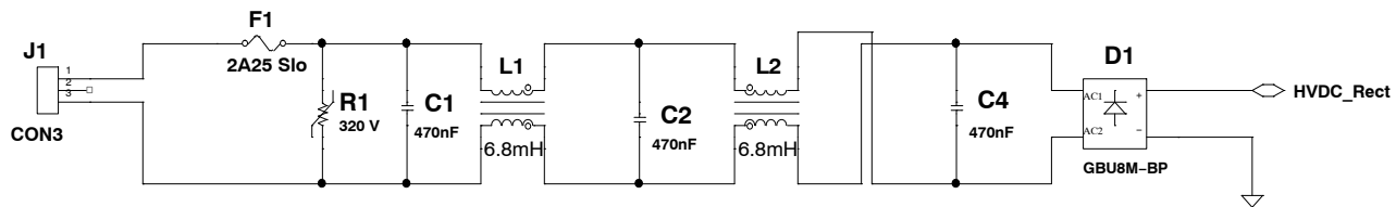
Figure 4. Input Circuit
