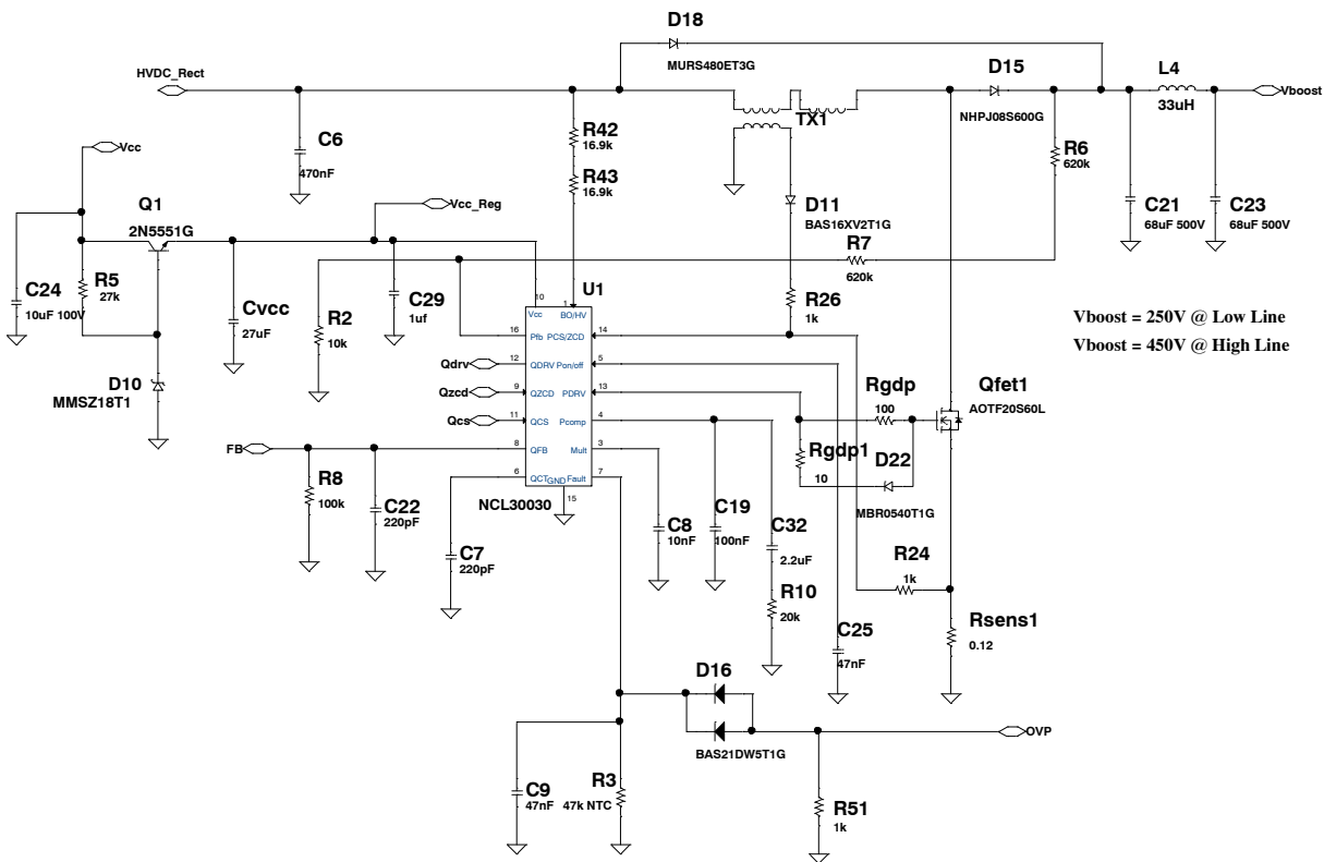
Figure 5. PFC Schematic
