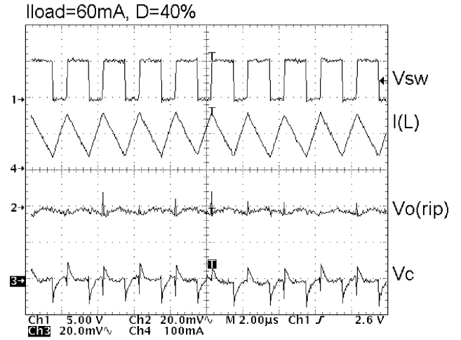
Figure 14. Minimum Load 500 kHz Operating Waveforms
