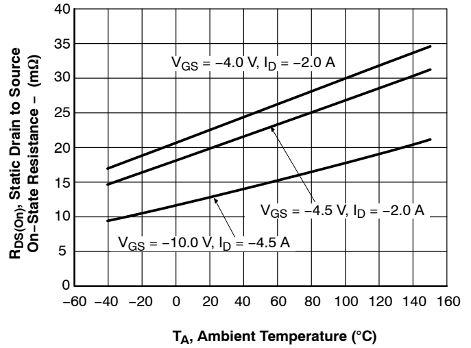
Figure 5. R_{DS(on)} - T_A
