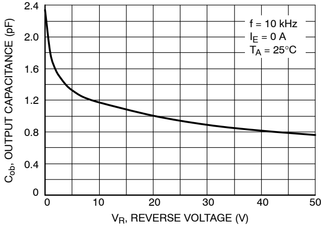
Figure 10. Output Capacitance
