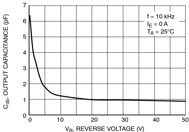
Figure 19. Output Capacitance
