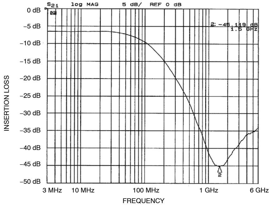
Figure 1. Insertion Loss vs. Frequency (FILTER1 Input to GND, CM1631-04DE)
