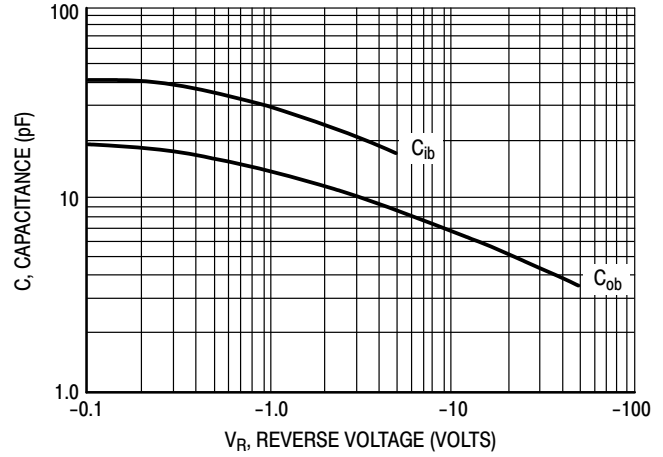
Figure 16. Capacitances
