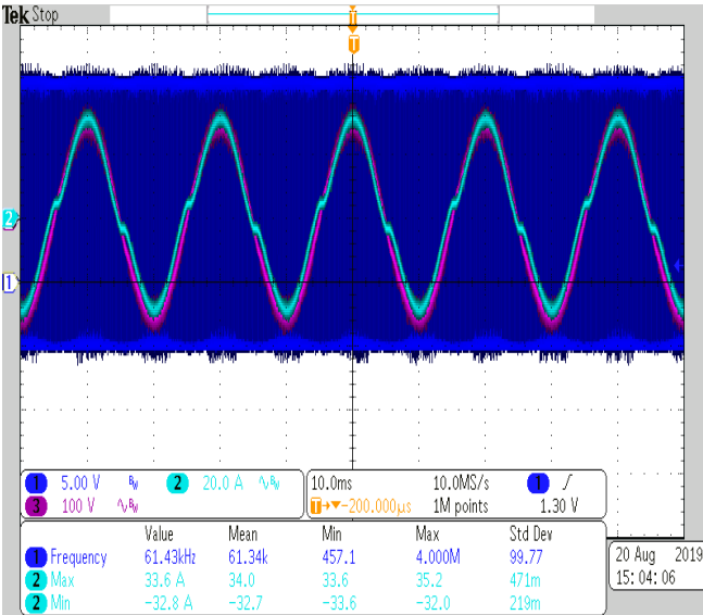
Figure 23. Vin = 110 Vac, Vo = 400 V, Iin = 20 A
