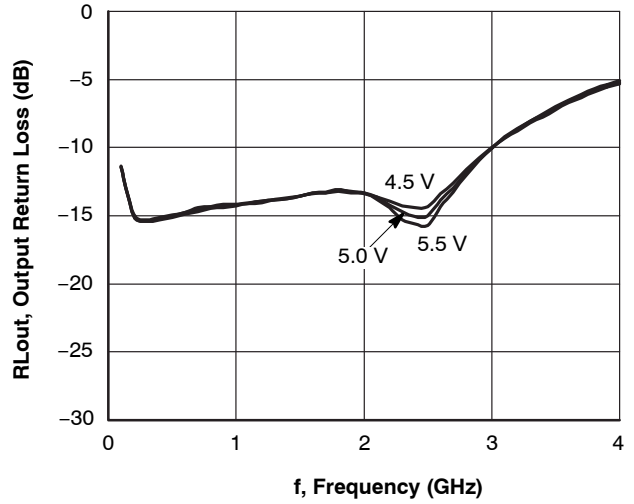
Figure 7. RL_{out} - f
