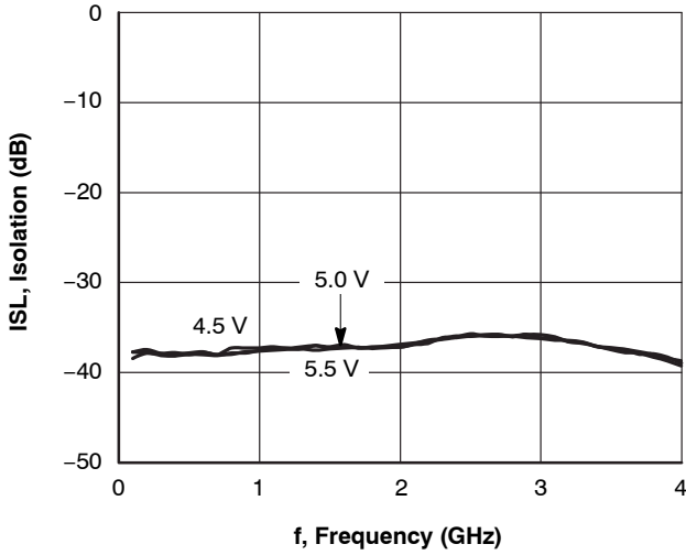
Figure 6. ISL - f
