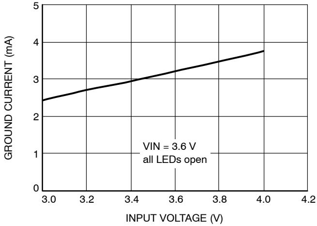
Figure 9. Ground Current vs. Input Voltage (1.5x Mode)
