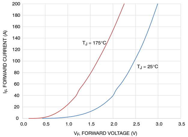
Figure 32. Typical Diode Forward Characteristics
