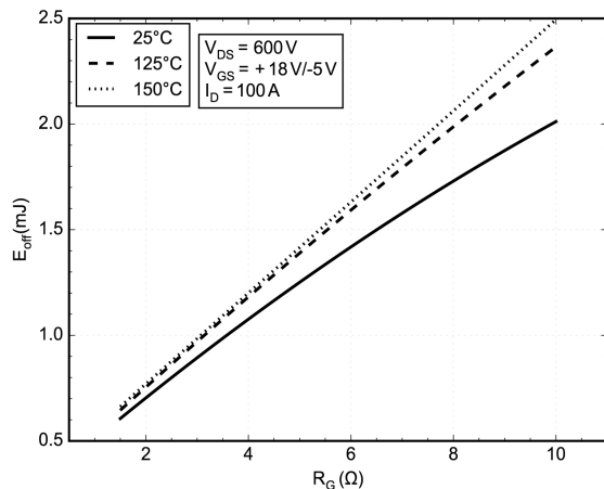
Figure 12. Typical Switching Loss E_{off} vs. R_G
