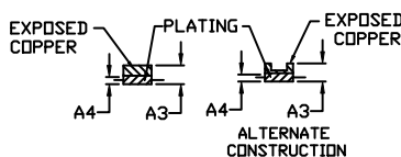
DETAIL B
