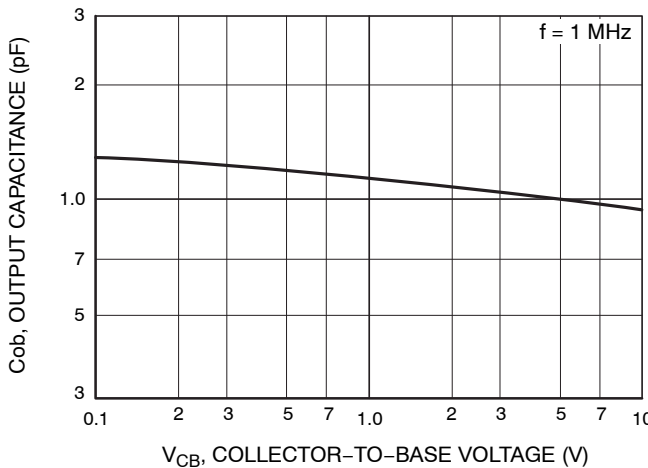
Figure 5. C_{ob} - V_{CB}
