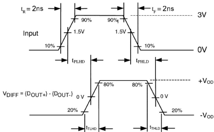
Figure 3. AC Waveforms
