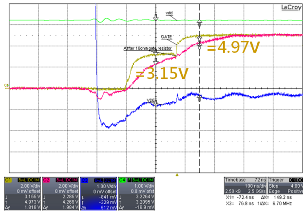
Figure 16. V_{OH} Level with C_{CP} = 10\text{ nF} (ch1: GATE pin; ch2: MOSFET Vgs; ch3 : VRAIN : ch4 : VDD)
