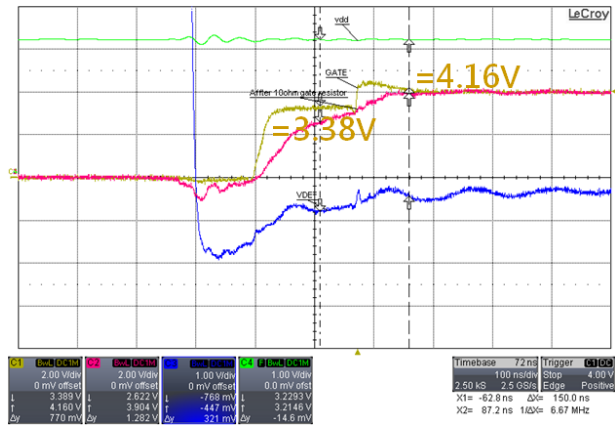
Figure 15. V_{OH} Level with C_{CP} = 2.2\text{ nF} (ch1: GATE pin; ch2: MOSFET Vgs; ch3 : VRAIN : ch4 : VDD)
