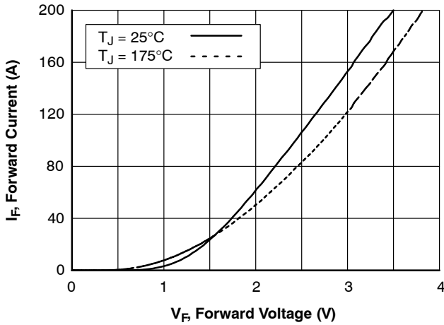
Figure 15. Forward Characteristics
