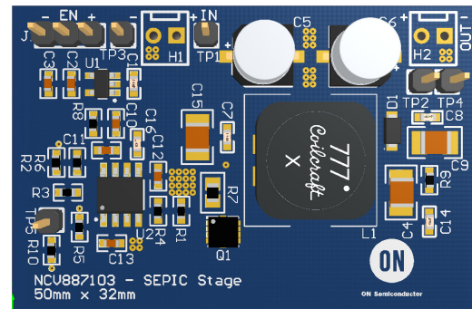
Figure 1. Reference Design PCB Print
