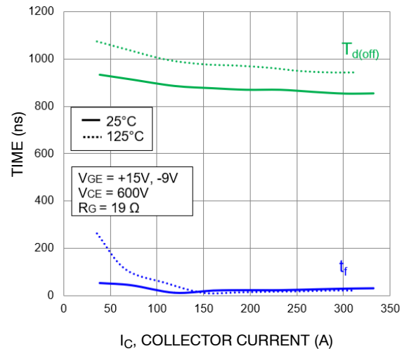
Figure 12. Typical Turn-Off Switching Time vs. IC
