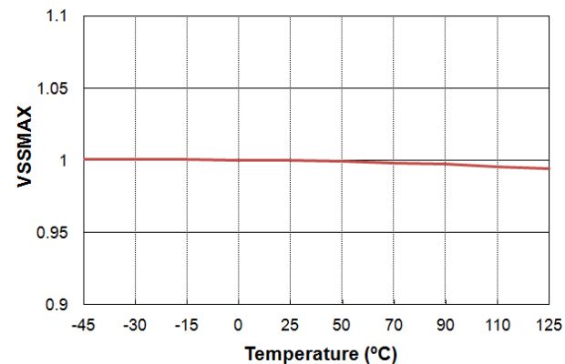
Figure 32. V SS,MAX vs. Temperature
