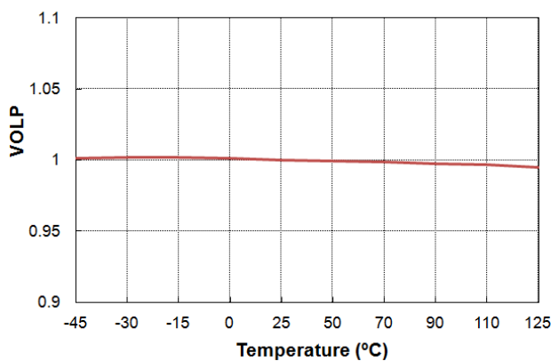
Figure 30. V OLP vs. Temperature
