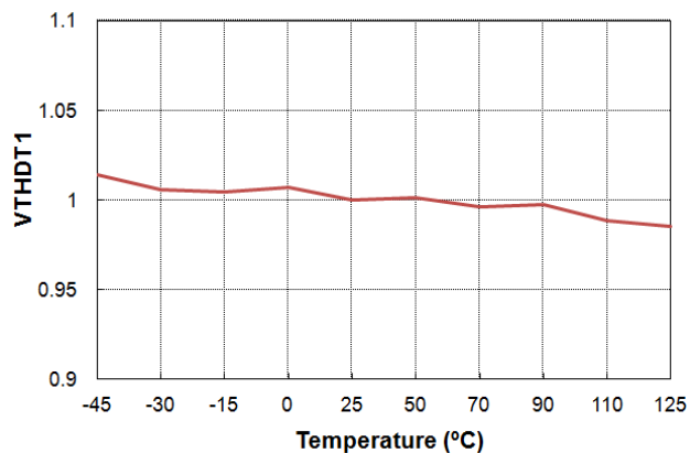
Figure 27. V THDT1 vs. Temperature
