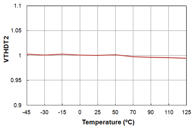
Figure 28. V THDT2 vs. Temperature
